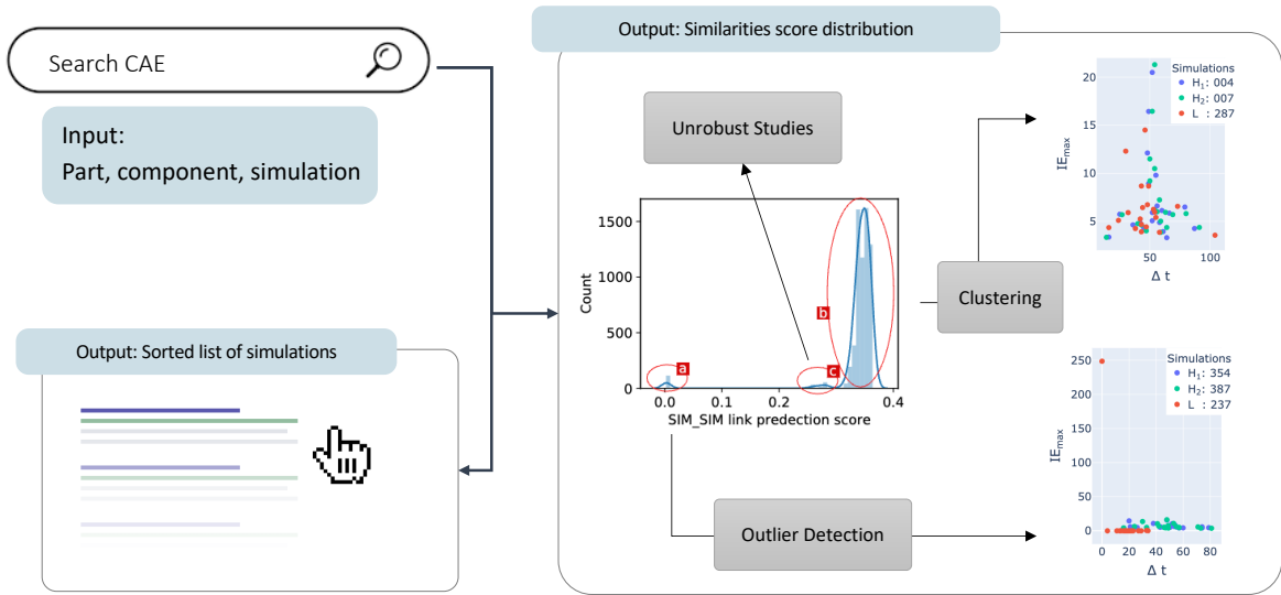
Figure 18: User workflow for simulations searchability.
