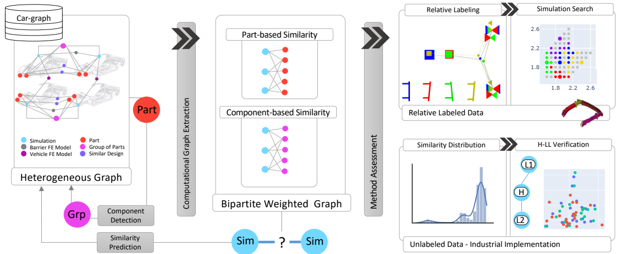
Figure 1: Similarity prediction workflow for relative labeled and unlabeled data. This workflow considers parts and part groups (components) and predicts the similarity based on two variants of a bipartite graph. The nodes' coloring in the heterogeneous graph reflects different node types.
