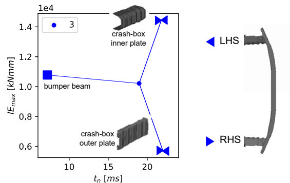
Figure 8: Energy diagram for the base simulation, number 3 in Section 3, considering five parts.
