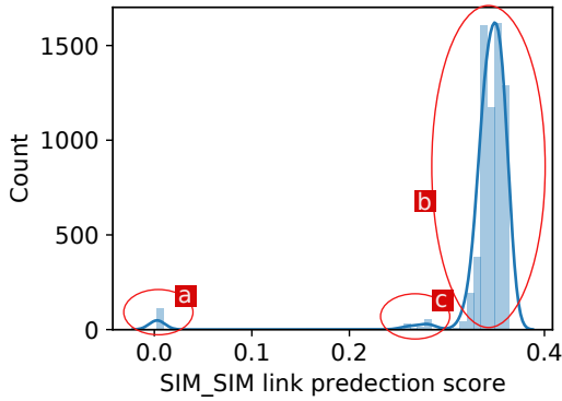
Figure 14: s_{trgt}^{++} link prediction histogram and estimated density for the foI load-case in the primary stage, CEVT data. (a), (b), and (c) highlights the three cluster of similarity distributions.
