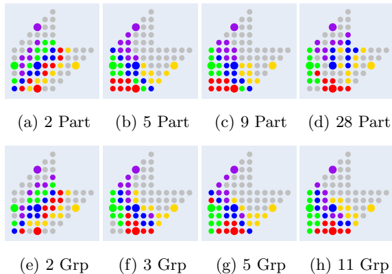
Figure 13: Comparing relative labeling of part-based (a)(b)(c)(d) with component-based (e)(f)(g)(h) while varying the number of (Part) and (Grp) nodes respectively. x-axis, y-axis, and coloring are the same as in Figure 12.
