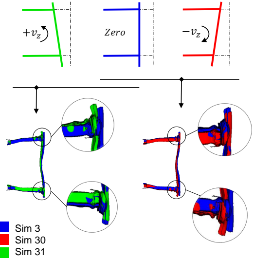
Figure 4: Defined relative label for crash mode based on Yaw axis rotation. FE simulations result follows the color coding of the crash modes.
