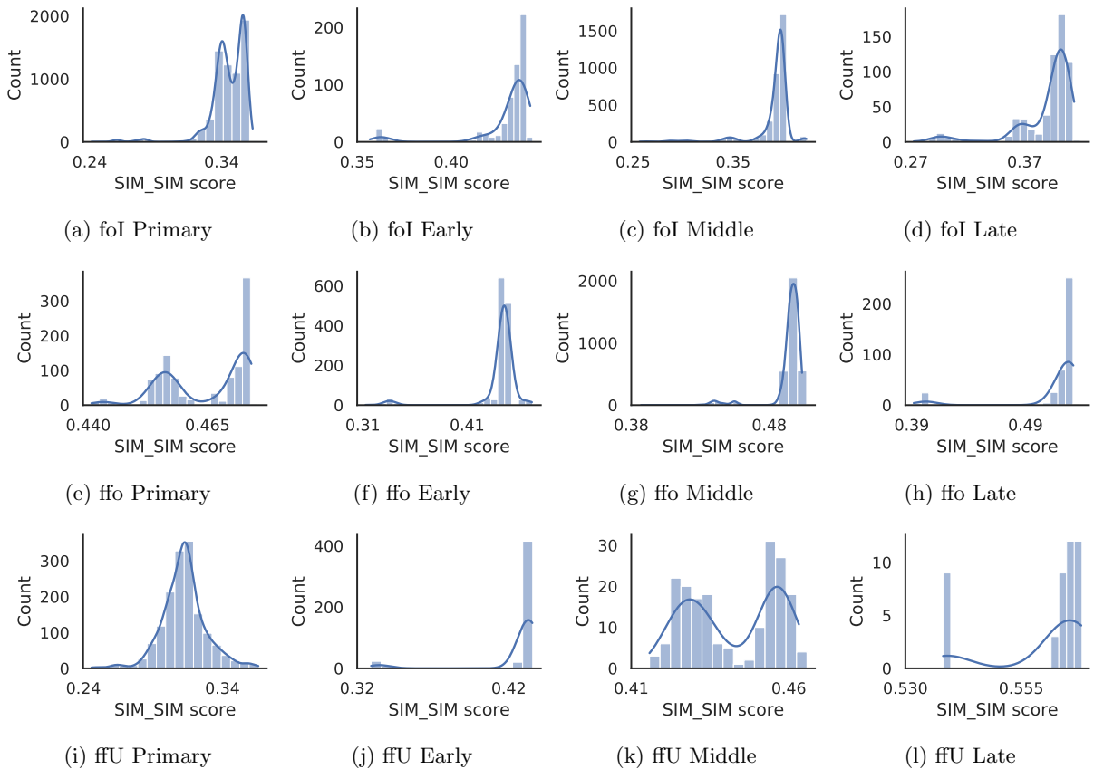
Figure 15: KDE plot for s_{tgt}^{++} prediction with 20 most energetic parts in three different load-cases full front overload (ffo), front oblique overlap (foI), and front small overlap (ffU) in four development stages, primary, early, middle and late that reflects the sequence of the stage, for more information look in Section 3 of [18]. The simulations with a maximal similarity less than 0.2, and therefore outliers, are removed.
