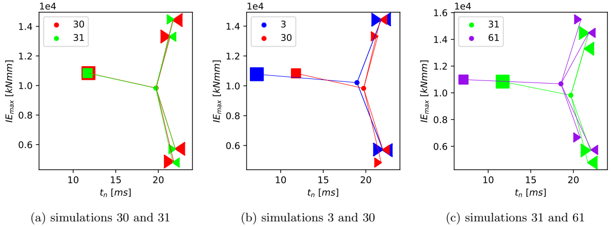
Figure 9: Energy diagram for selected simulations from Section 3.
