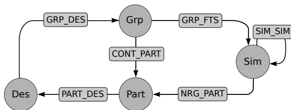
Figure 10: Graph data schema used for simulations similarity prediction, full schema available in [17].
