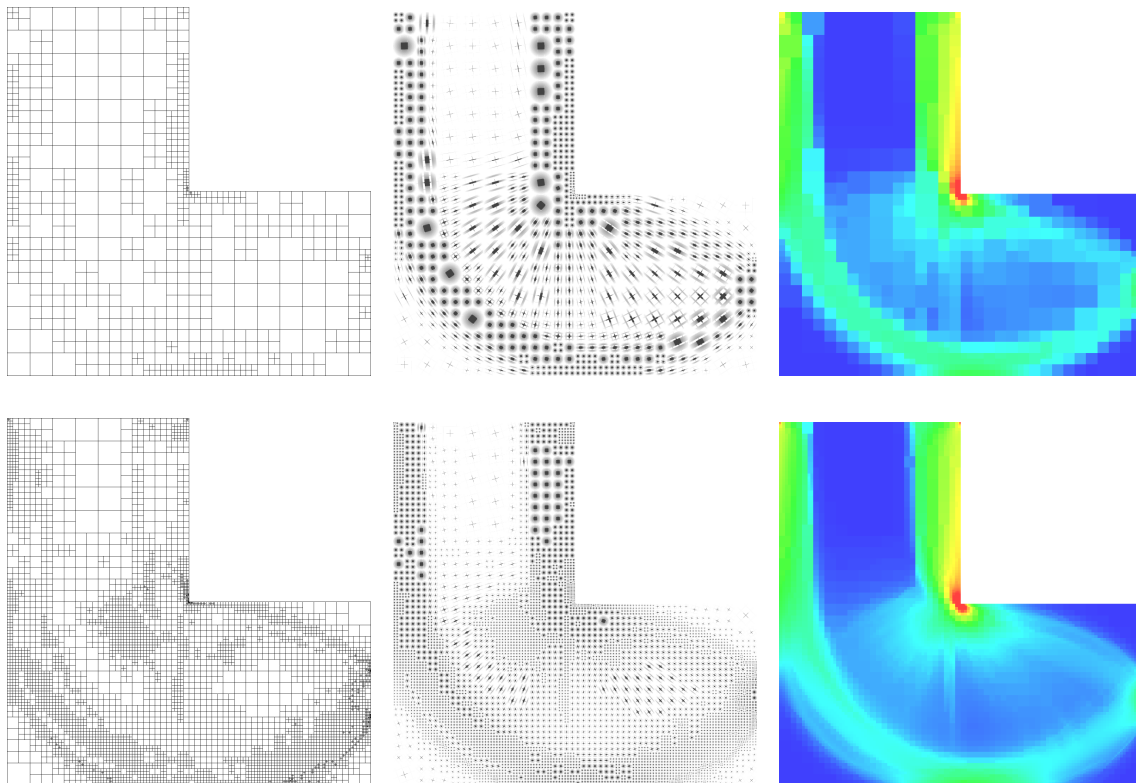
Figure 7: For the L-shaped domain after 4 / 9 refinement steps: adaptively refined grid; visualization of the two-scale model as in Figure 3; von Mises stress with color coding as in Figure 3 for values in [0, 4] .
