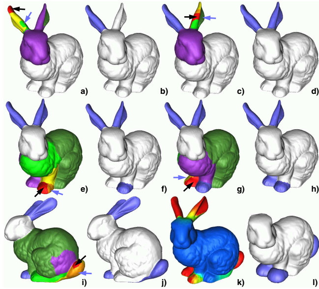
Fig. 12 Application 1: In ten clicks, five features (ears, front paws, tail) are selected (a-j). Next, the handle and the edited surface are shown (k,l)
