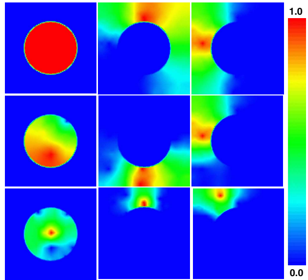
Fig. 5 For a simple second order differential operator on a planar domain, algebraic multigrid basis functions are depicted on different scales (upper row: coarsest scale, middle row and lower row successively finer scales). The basis functions clearly reflect the ring type feature region encoded in the operator.
