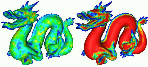
Fig. 7 The zero moment and the combined moment feature classifiers are compared on a triangular mesh. The combined classifier detects significantly more robustly the surface edges.
