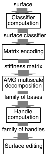
Fig. 2 Steps of the multiscale surface editing method
