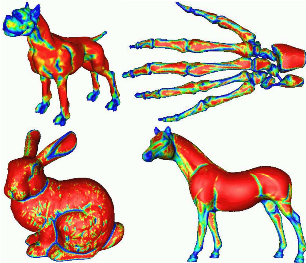
Fig. 8 For different triangular surface meshes we show the local feature classification result using a color coding for the classifier \mathcal{C}^{0,1}(\cdot) .
