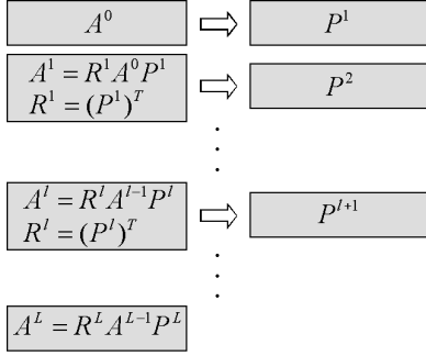
Figure 2: General AMG construction. From the fine scale matrix A^0 input, AMG computes prolongations P^l , restrictions R^l , and coarse scale matrices A^l on successively coarser scales l = 1, \dots, L .
