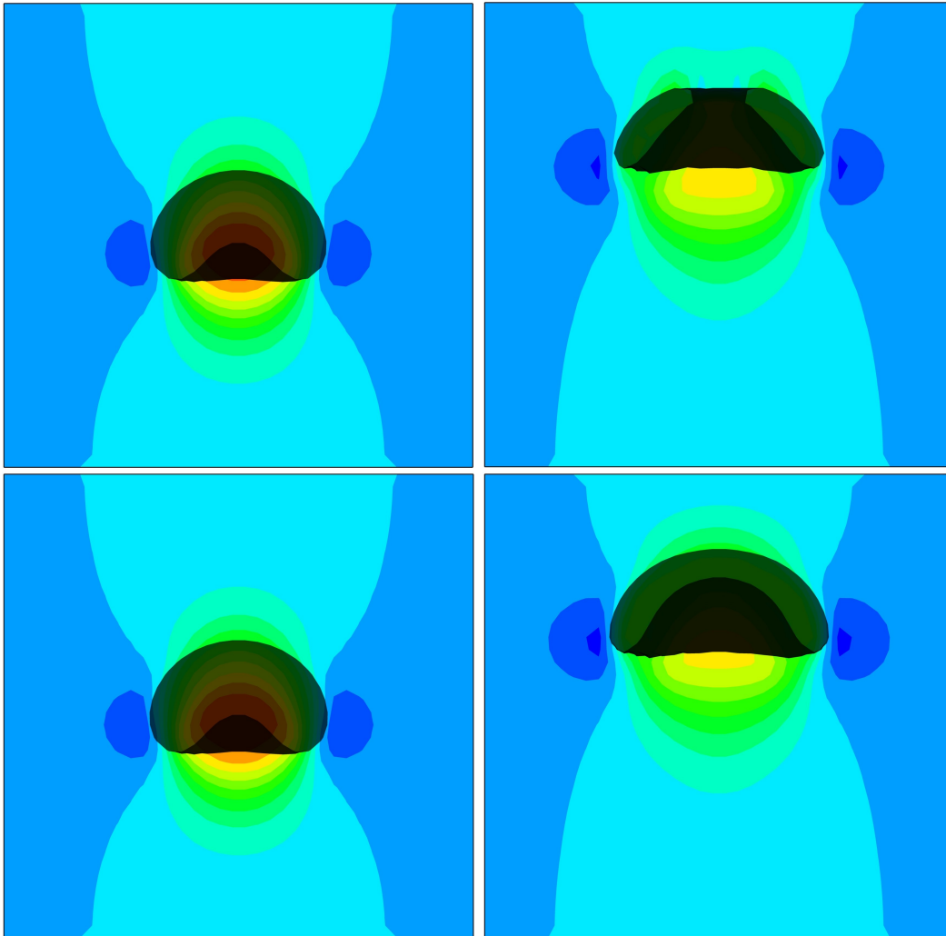
Figure 7. Rising bubble without (upper row) and with (lower row) fixed point iteration for improved mass conservation at times t = 0.075s (left column) and t = 0.15s (right column) for h = 1/37 . Depicted is a semi-transparent iso-surface of the zero-level set and a contour plot of the v-velocity along the center plane.
