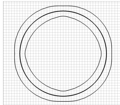
Figure 4. Numerical smoothing region defined in (33) with c_\alpha = 2 for a spherical droplet.
