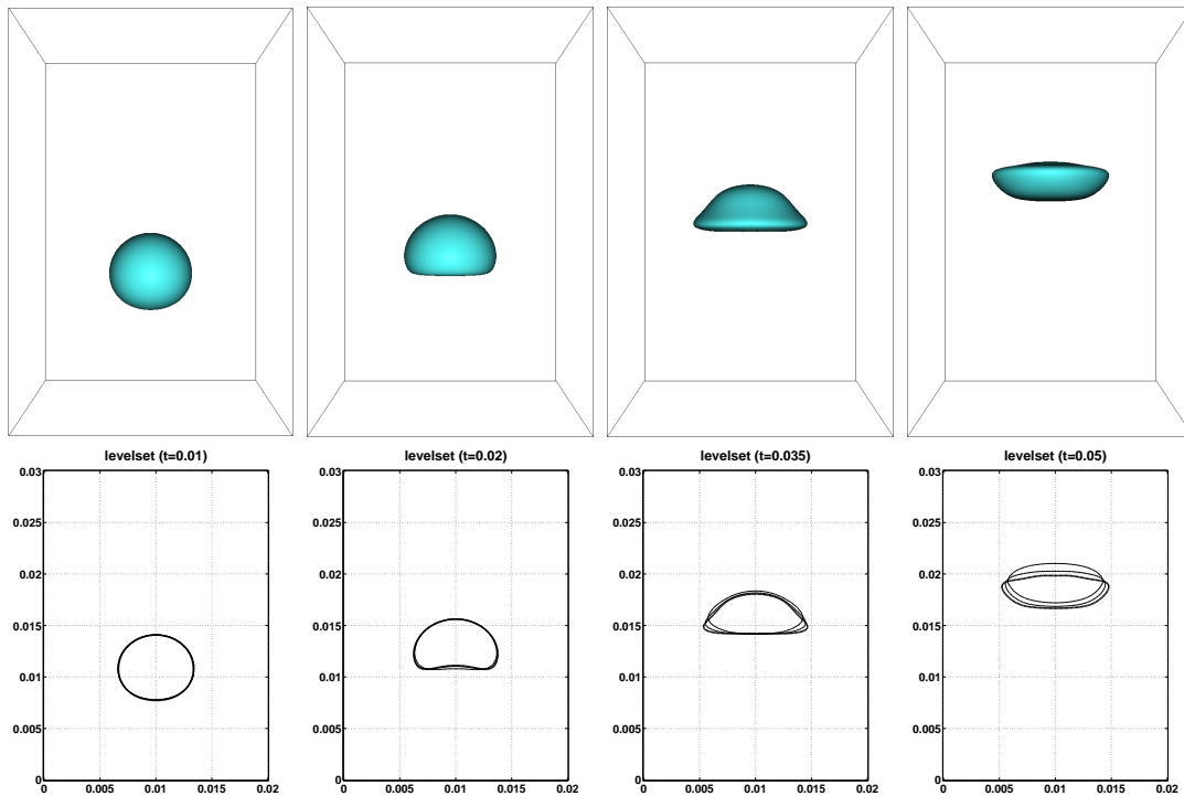
Figure 8. Air bubble rising in water at times t = 0.01s , 0.02s , 0.035s , and 0.05s (left to right). Depicted in the top row are the interface positions for mesh-width = (1/160, 1.5/240, 1/160) . On the bottom row we give the intersections of the interface with the center plane of the computational domain for the mesh-widths = (1/40, 1.5/60, 1/40) , (1/80, 1.5/120, 1/80) , and (1/160, 1.5/240, 1/160) (bold line corresponds to finest resolution).
