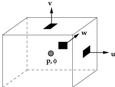
Figure 3. Location of variables in a staggered grid cell.
