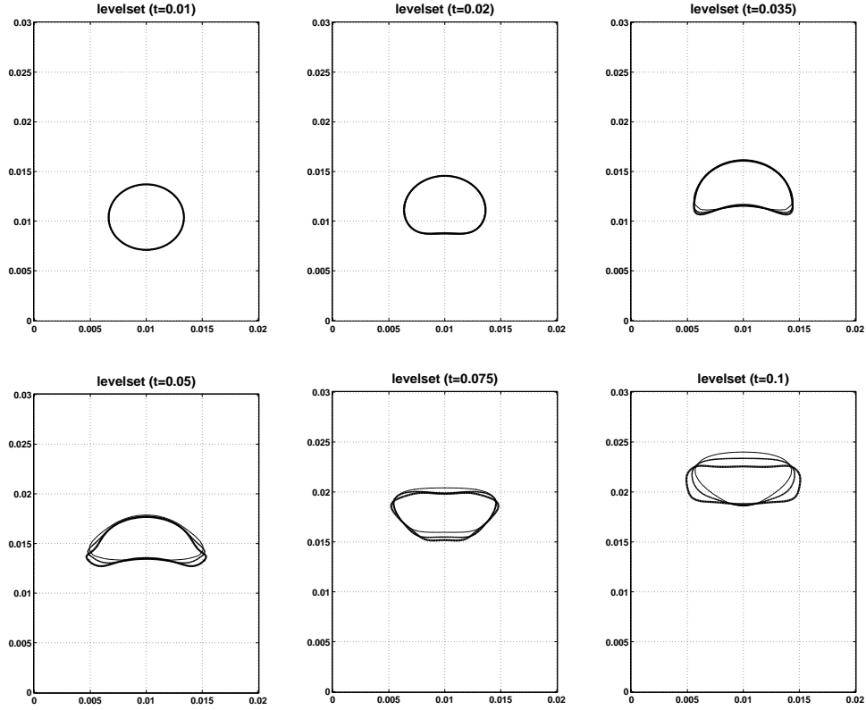
Figure 9. Quasi 2D air bubble rising in water at times t = 0.01s, 0.02s, 0.035s, 0.05s, 0.075s and 0.1s . We give the intersections of the interface with the center plane of the computational domain for the mesh-widths = (1/40, 1.5/60, 1/4) , (1/80, 1.5/120, 1/8) , and (1/160, 1.5/240, 1/16) (bold line corresponds to finest resolution).
