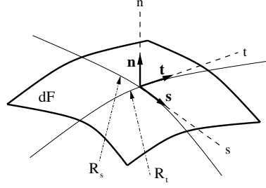
Figure 1. Curvature for surface tension computation.
