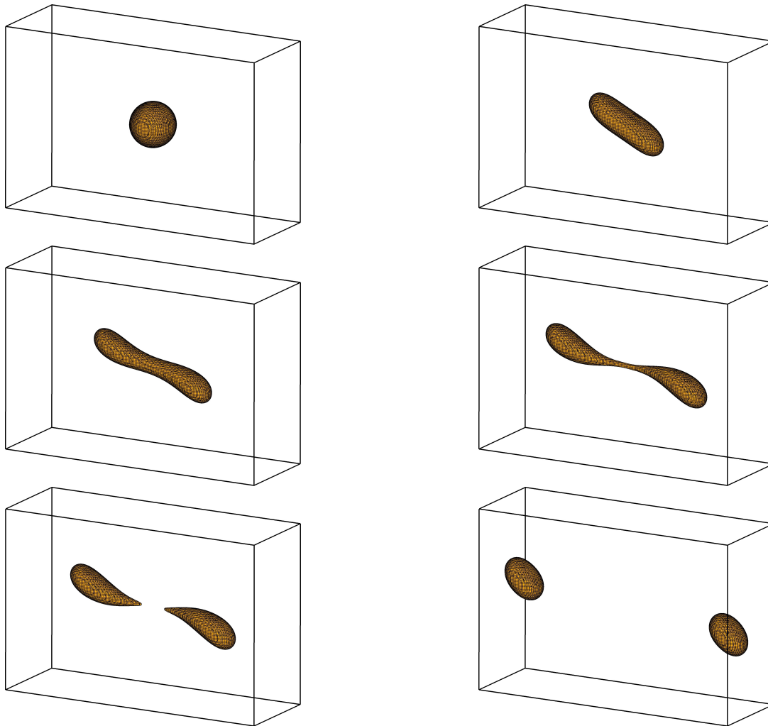
Figure 13. Instationary results obtained for the parameter setting (Ca, Re) = (0.15, 15) . Depicted are the configurations of the free surface at the dimensionless times t^* = 0 , t^* = 334.8 , t^* = 379.2 , t^* = 396.0 , t^* = 397.2 , t^* = 416.40 (upper left to lower right). The simulation domain is 3 \times 1 \times 2 and the droplet has a radius of r = 0.25 . The mesh-width is (3/192, 1/64, 2/128) .
